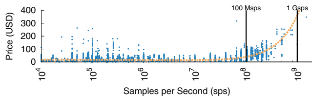
Fig. 4: ADC price versus sampling speed. We scrape all 9,716 of the available ADCs from DigiKey and collect the price per unit for the best bulk rate, discarding products only available in very small quantities (those with no bulk option available). There exists a super-linear relationship between price and sampling rate above about 100 Msps, which is required for traditional UWB anchors. Careful selection of ADC sampling rate is necessary for cost-effective anchor design.
