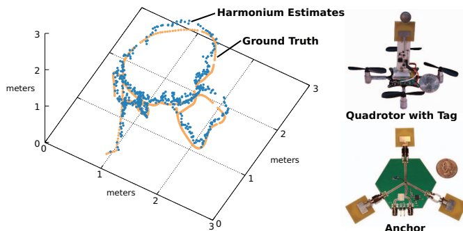
Fig. 1: A Harmonium system reconstructs the flight path of a 19 g quadrotor in a 3\times 3\times 3 m space at a 19 Hz update rate using four anchors and a tag that is small ( 1.5\text{ cm}^3 ), low-cost ($4.50), lightweight (3 g), and low-power (75 mW). Ground truth is acquired using the commercial OptiTrack optical motion capture system. Harmonium tracks the path with 14 cm median error and 46 cm error at the 95th percentile.
