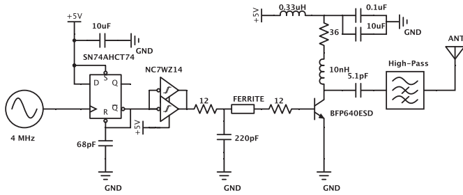
Fig. 6: Tag circuit diagram showing the detailed interconnection between the oscillator, monostep generator, and BJT transistor. Additional passives are necessary for FCC-compliant pulse shaping. Total tag cost in modest quantity is approximately $4.50 per tag.
