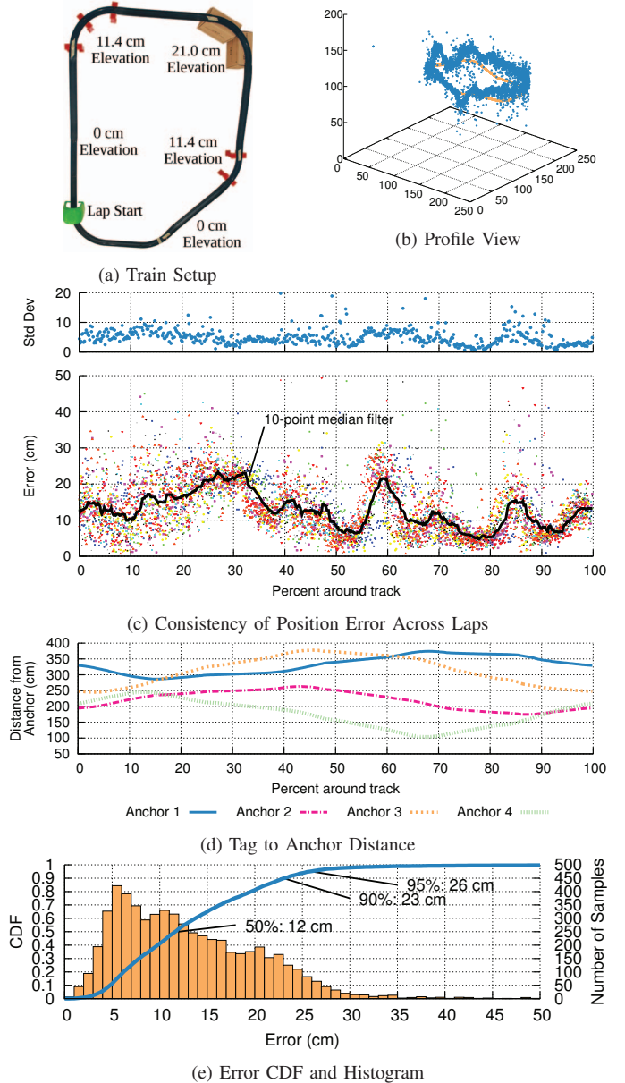
Fig. 10: Point-cloud of location estimates and CDF of errors tracking ten laps of a model train around a track. Errors are consistent in space, implying a physical root cause.
